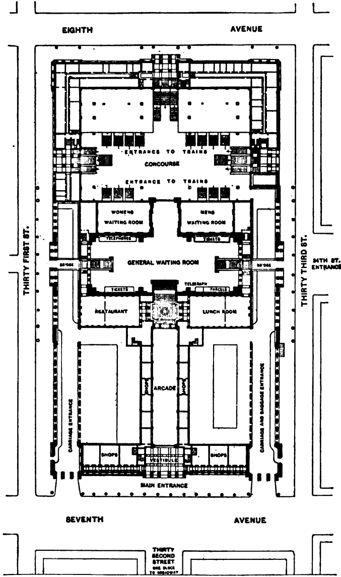
FIG. 112.—Street floor plan, Pennsylvania Terminal.
