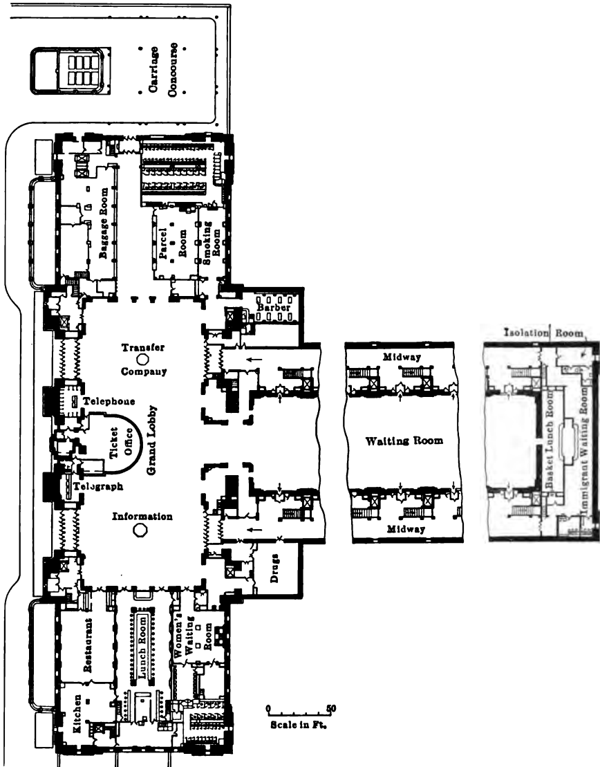
FIG. 61.—Floor plan of Union Station, Kansas City, Mo.
