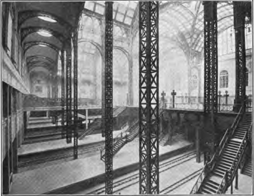
FIG. 115.—Train shed of Pennsylvania Station, New York.
