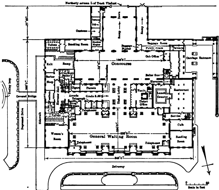
FIG. 47.—Floor plan of Michigan Central Station, Detroit.
