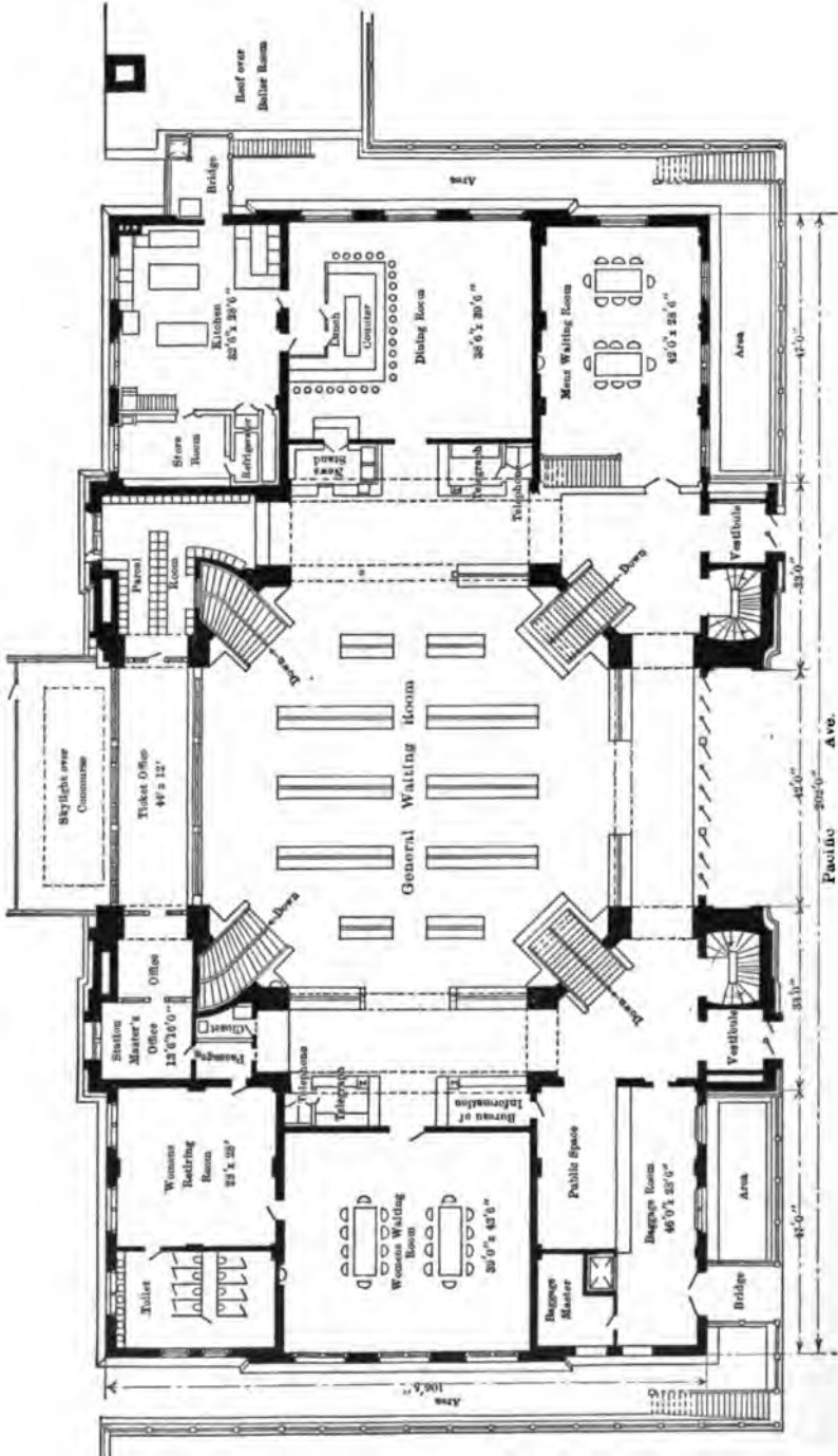
FIG. 65.—Plan of Northern Pacific Station, Tacoma, Wash.
