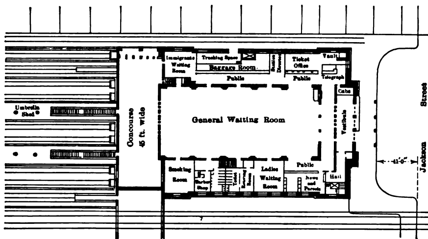
FIG. 83.—Main floor plan of Oregon-Washington Station, Seattle.
