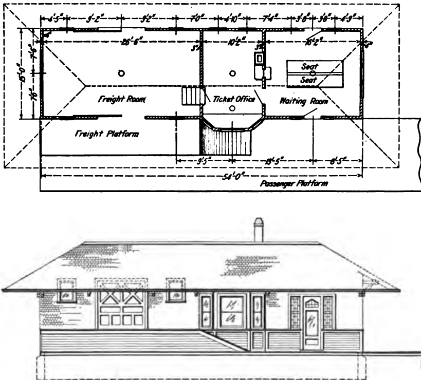
FIG. 172.—New Haven standard combination station, plan and elevation.
