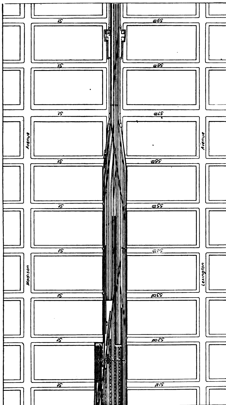
FIG. 31B.—Plan of tracks and approaches to Grand Central Terminal, New York—lower level.
