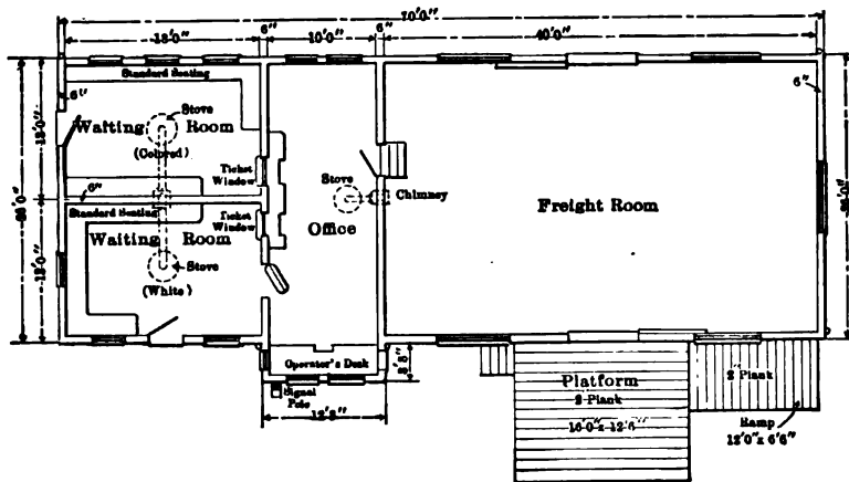
FIG. 167.—Plan of standard combination station on Virginian.
