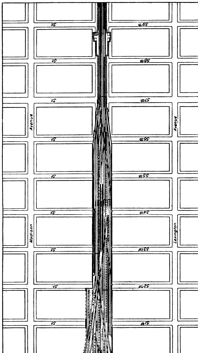
Fig. 31A.—Plan of tracks and approaches to Grand Central Terminal, New York—upper level.
