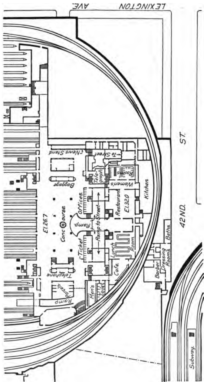
FIG. 123.—Floor plan of Grand Central Terminal, express train concourse and suburban concourse levels.
