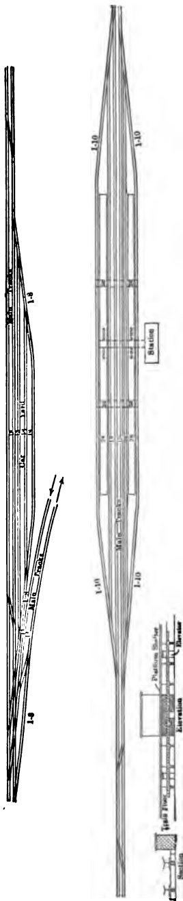
FIG. 39.—Typical track layout for through station, American Railway Engineering Association.
