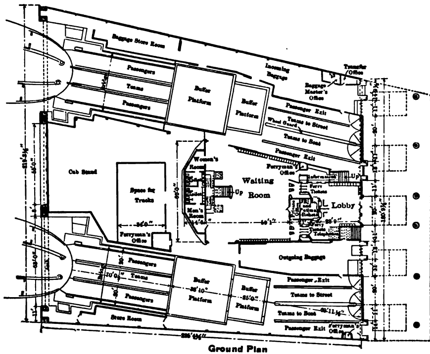
FIG. 101.—Erie Station at West 23rd Street, New York.
