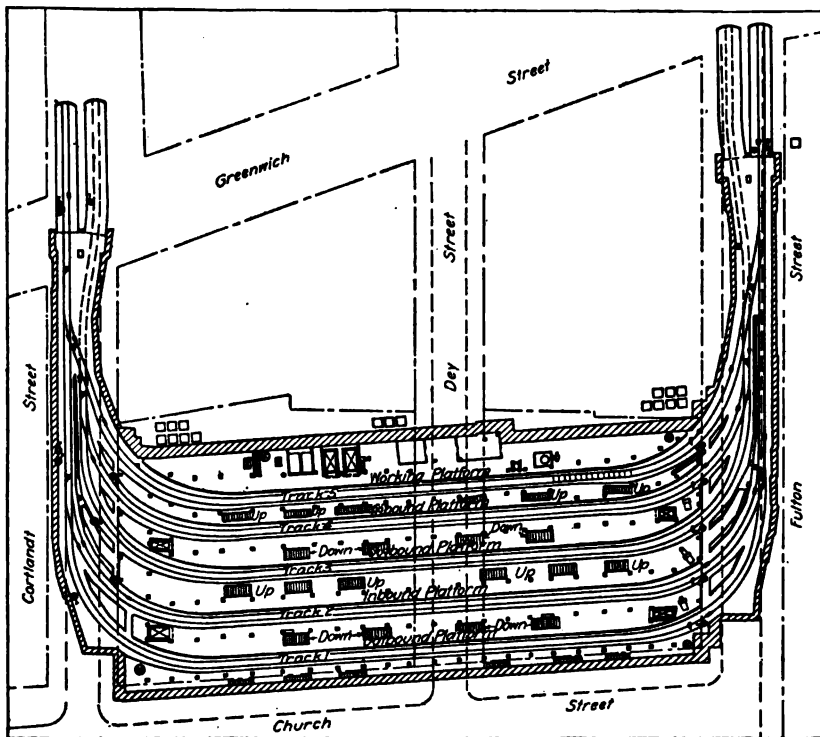
FIG. 118.—Track layout of the Hudson & Manhattan Station.
