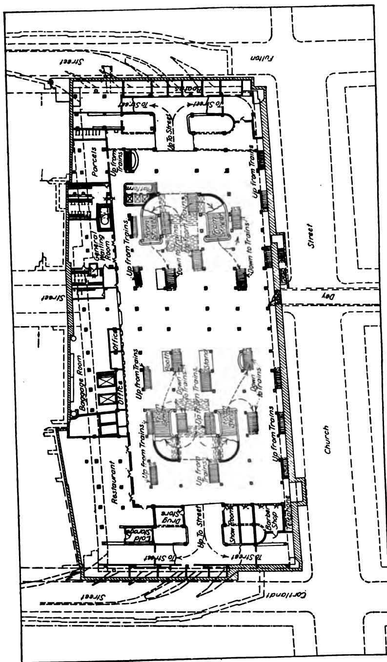
FIG. 119.—Plan of concourse—Hudson &amp; Manhattan Station.
