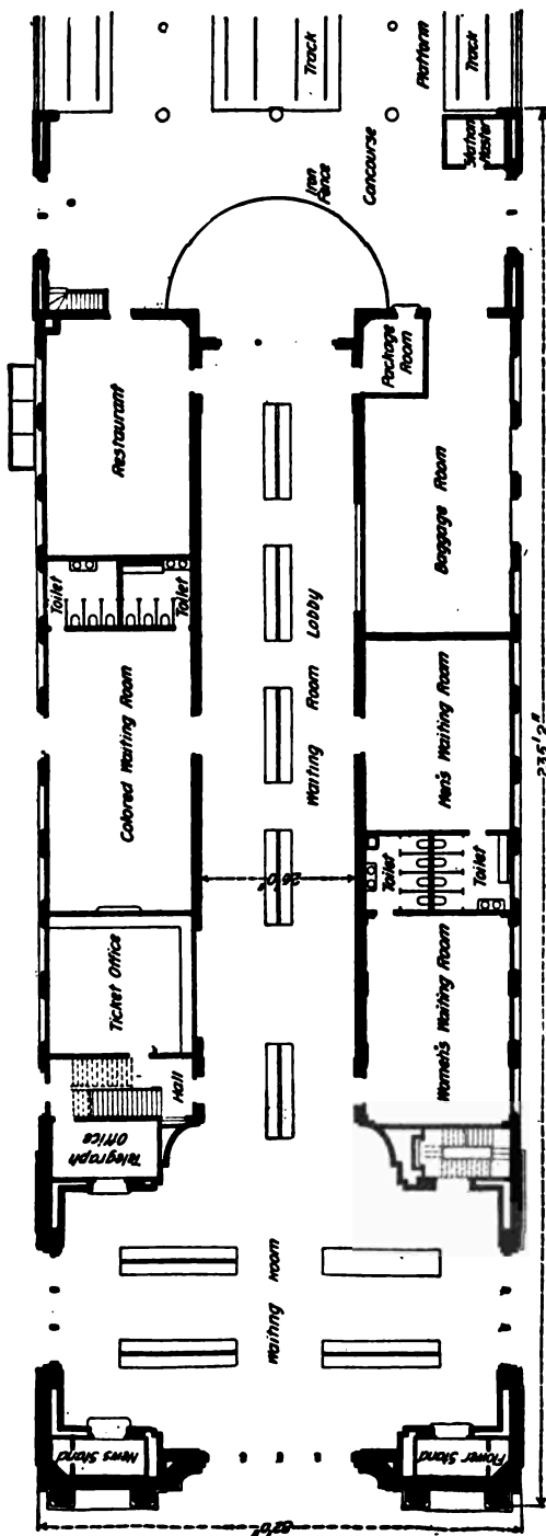
FIG. 80.—Plan of New Orleans Union Station.
