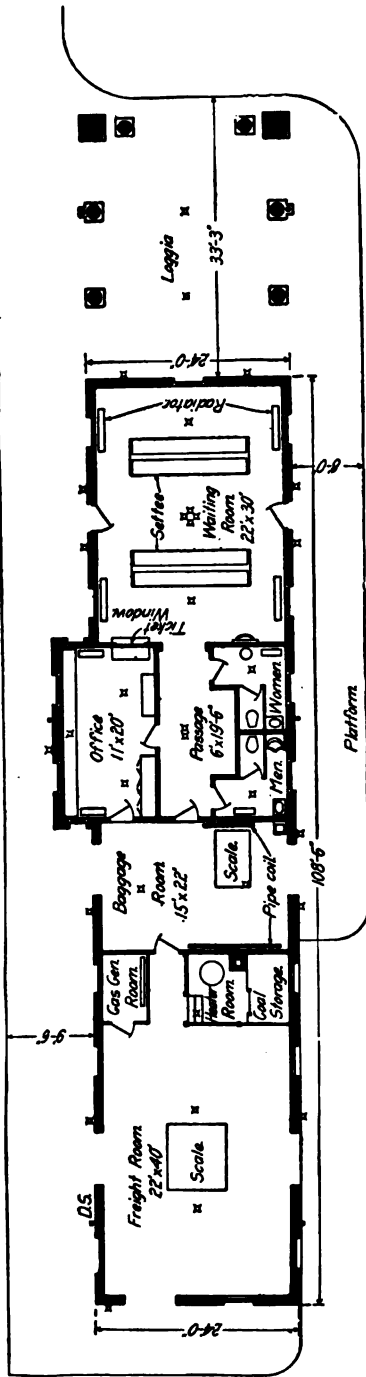
DL&W Combination Station with Separate Freight and Baggage Rooms Fig. 169.—Plan of combination station, Lackawanna.
