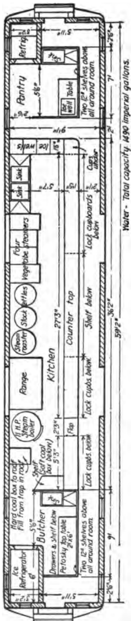
FIG. 220.—Canadian Pacific commissary kitchen car.
