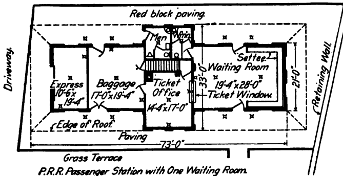
FIG. 158.—Plan of small station, Pennsylvania Railroad.
