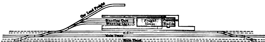
FIG. 171.—Berg's typical combination station.
