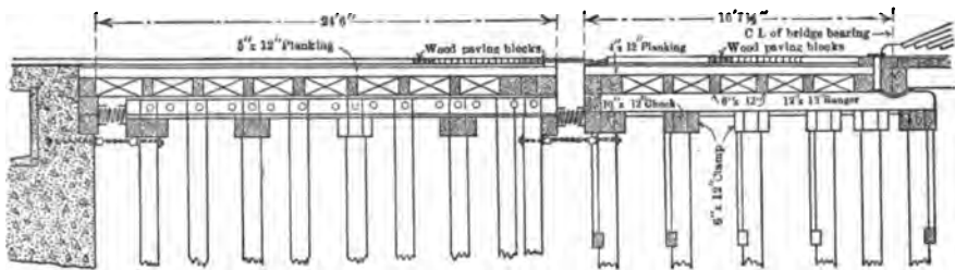
FIG. 100.—Details of buffer platform of ferry slip.
