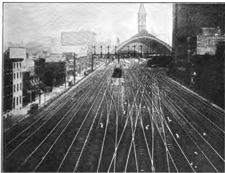
FIG. 29.—Leads to Broad Street Station, Philadelphia.
