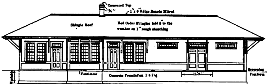
FIG. 166.—Elevation of combination station on Virginian.
