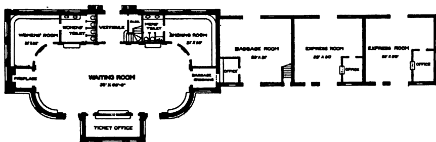
FIG. 42.—Plan of station at Grand Junction, Col.
