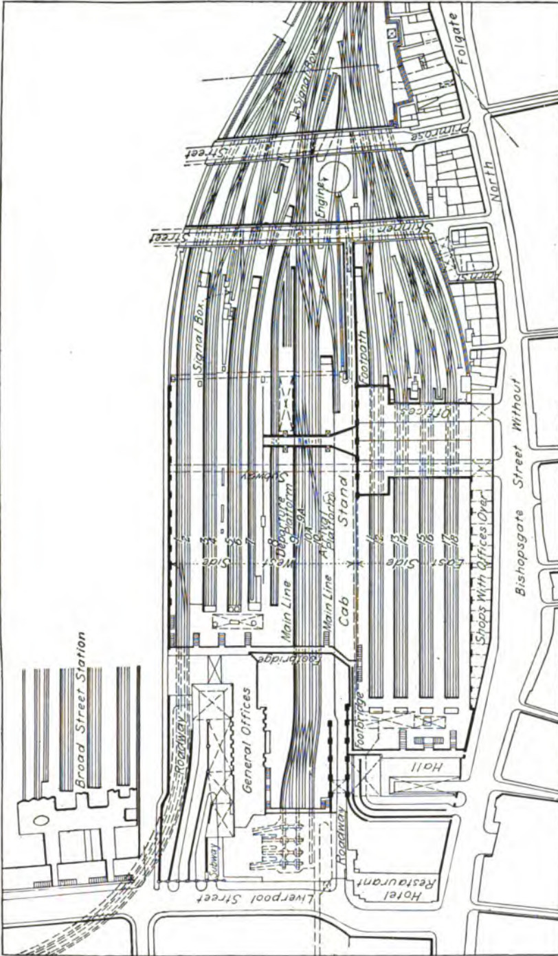
FIG. 177.—Plan of Liverpool Street Station, the busiest in London.
