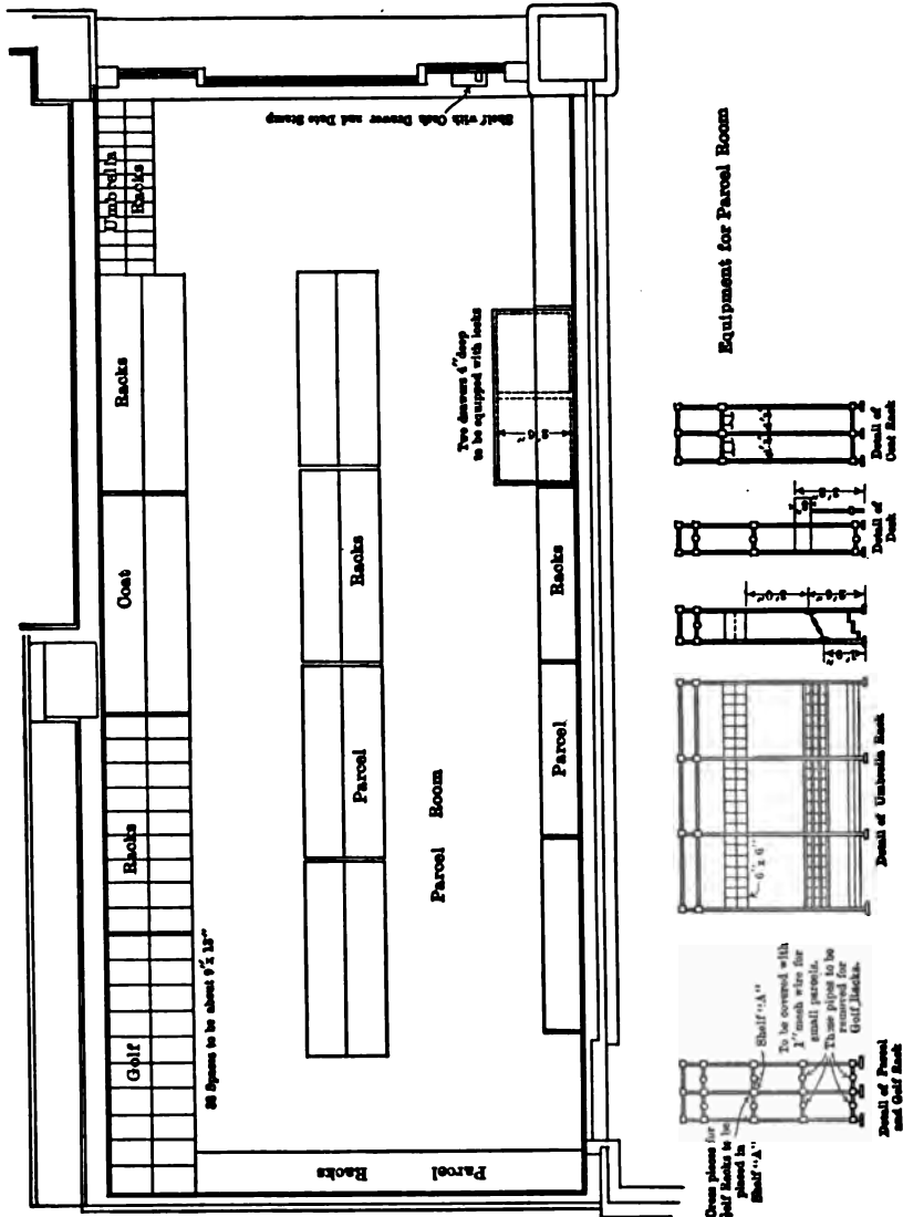
Fig. 143.—Plan of parcel racks in busy parcel room.
