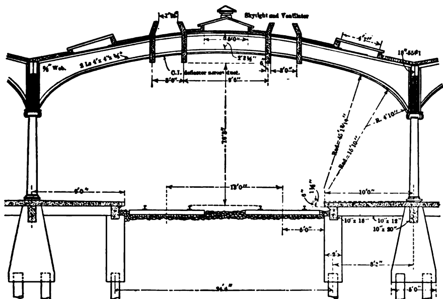
FIG. 23.—Details of Bush train shed in Central of New Jersey Station.
