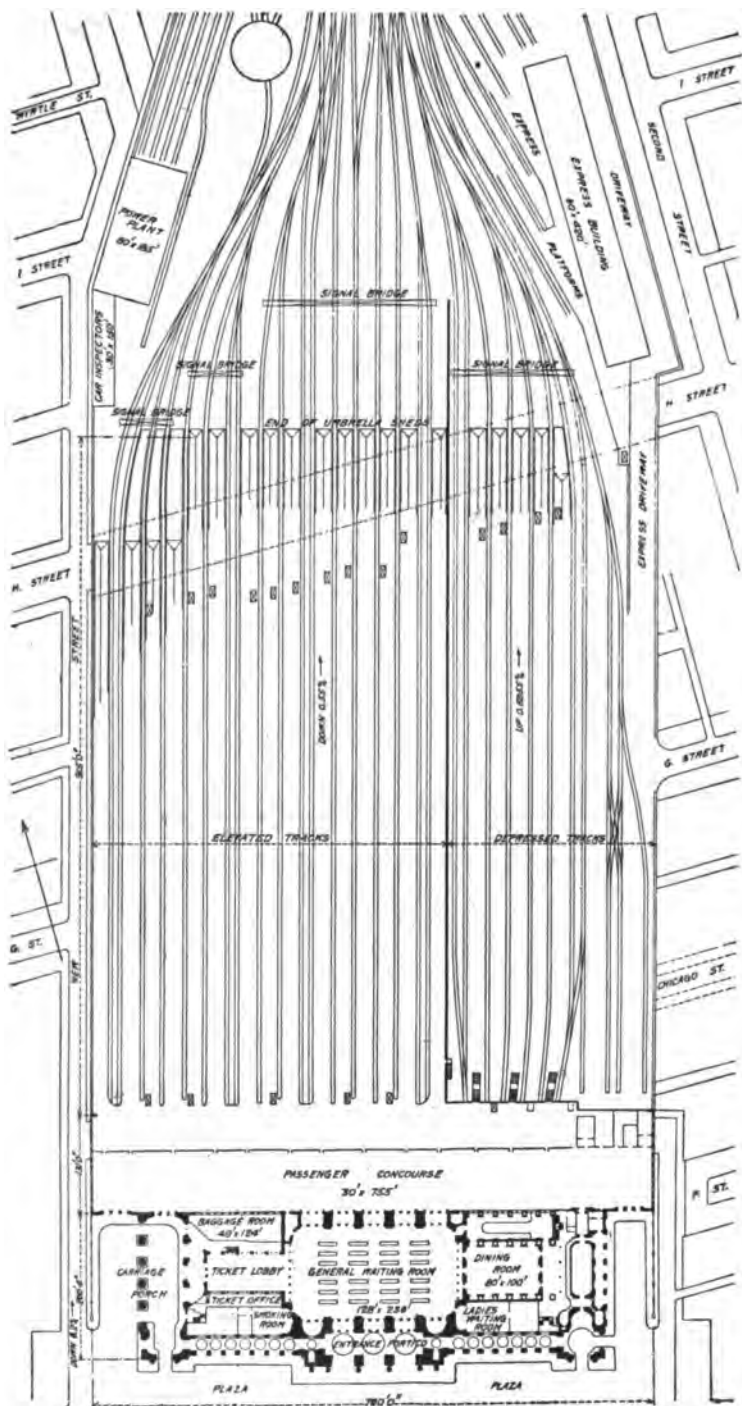
FIG. 77.—Plan of Union Station, Washington, D. C.
