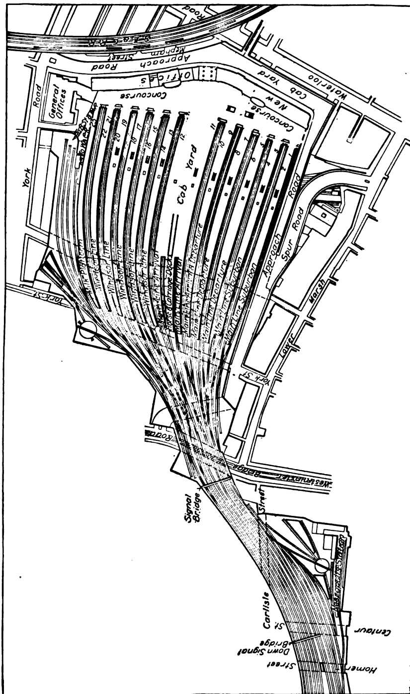
Fig. 176.—General plan of Waterloo Station. Tracks 1 to 6 and 16 to 21 are equipped for electric operation.
