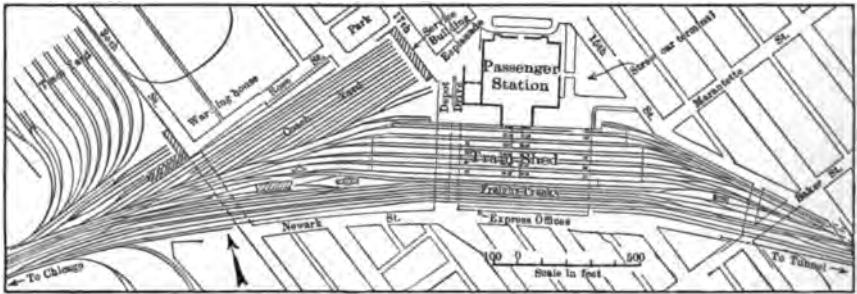
FIG. 145.—General plan of Michigan Central Station, Detroit, showing location of coach yards.
