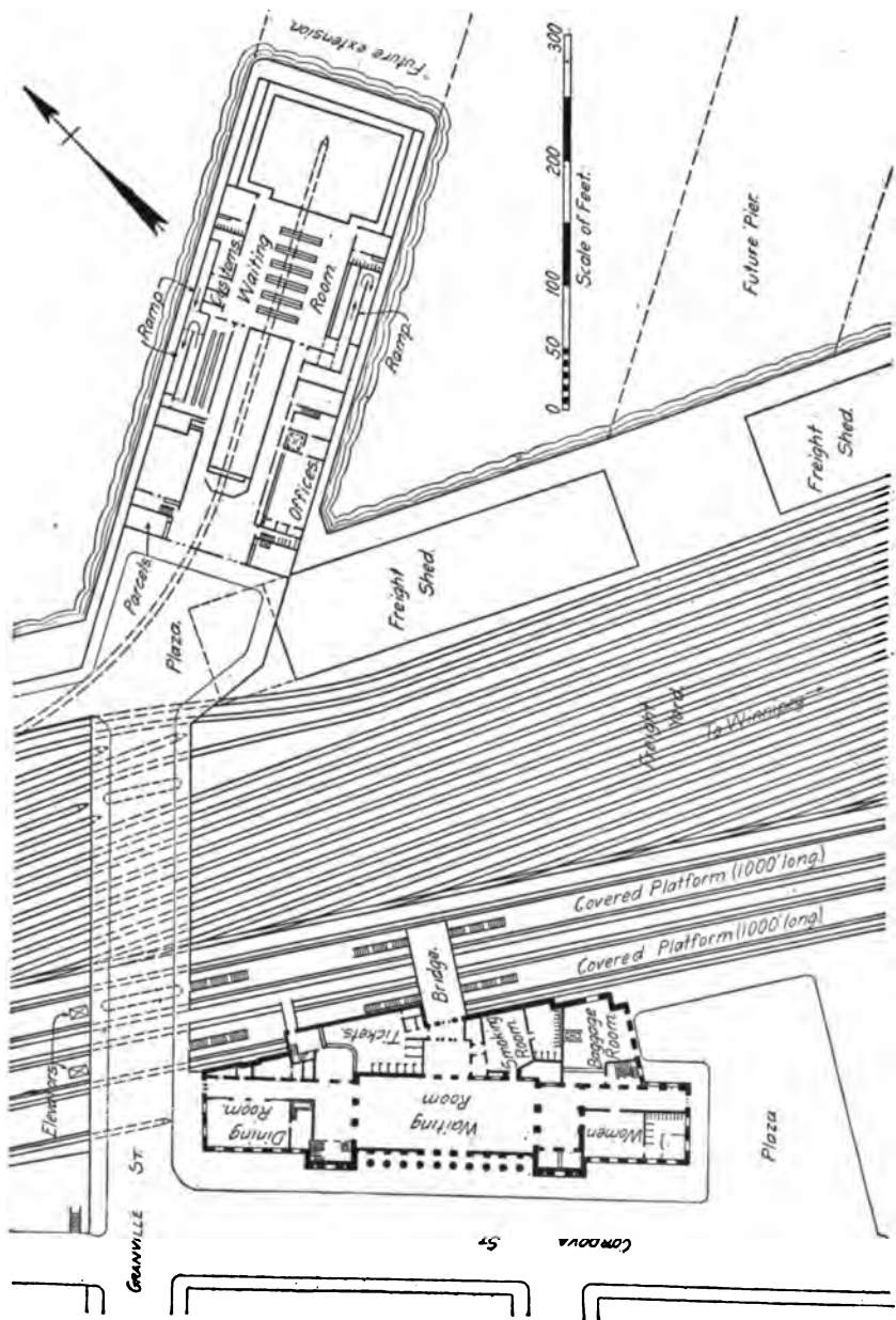
FIG. 107.—Canadian Pacific Terminal at Vancouver.
