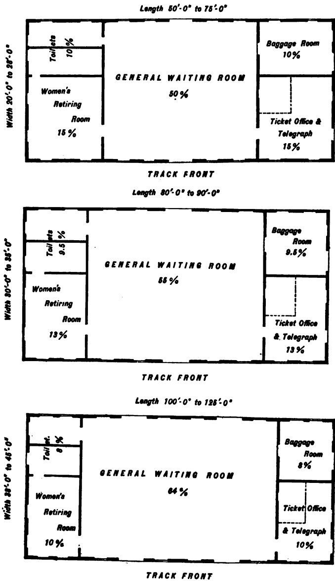
FIG. 154.—A. R. E. A. standard plans for small stations.
