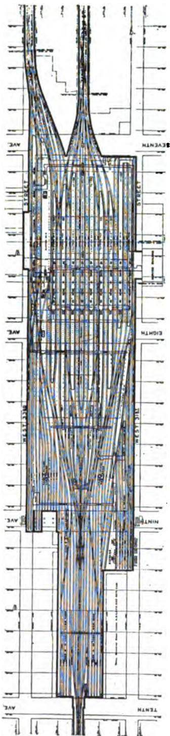
FIG. 111.—Track layout of Pennsylvania Terminal, New York.
