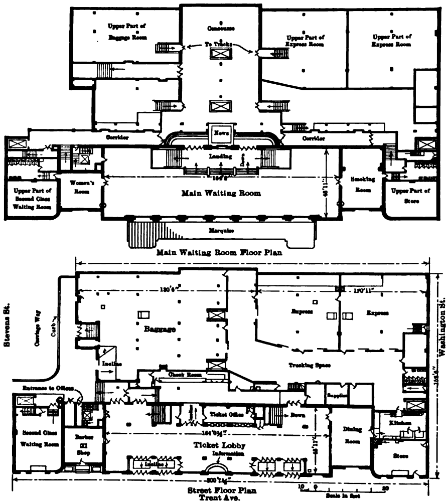
FIG. 56.—Plan of Oregon-Washington Station, Spokane.
