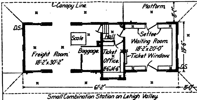
FIG. 170.—Plan of combination station, Lehigh Valley.
