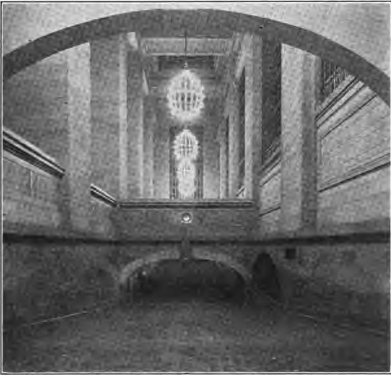
FIG. 125.—Ramps to suburban concourse, Grand Central Station.
