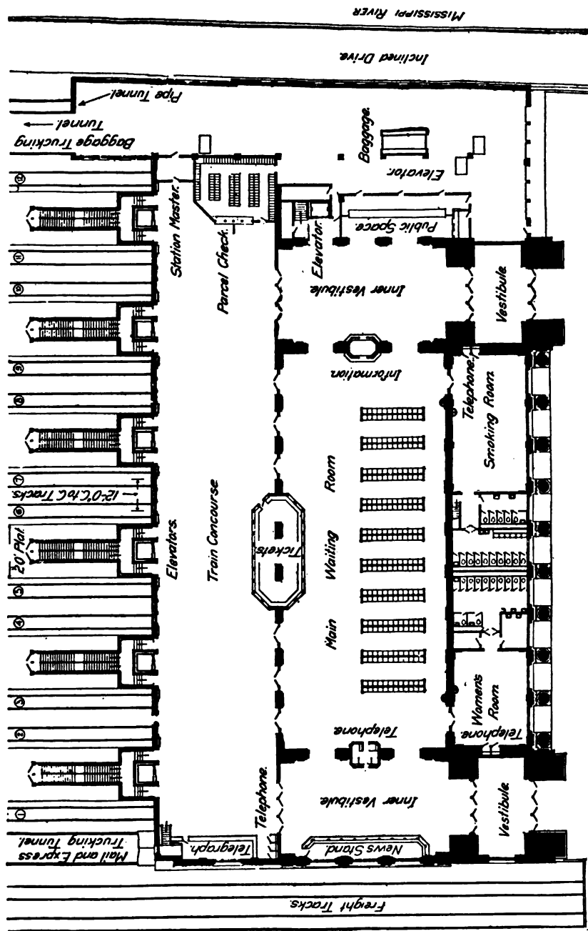
Fig. 66.—Great Northern Station at Minneapolis—floor plan.
